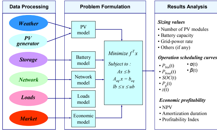
Figure 2. Overview of sizing and multi-sources management optimization algorithm.
