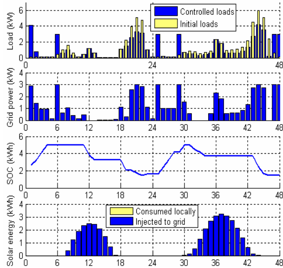
Figure 11. Operation plan for installation with 40% subsidies.
