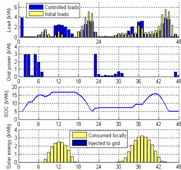
Figure 19. Operation plan for energy cost of 30 c€/kWh.
