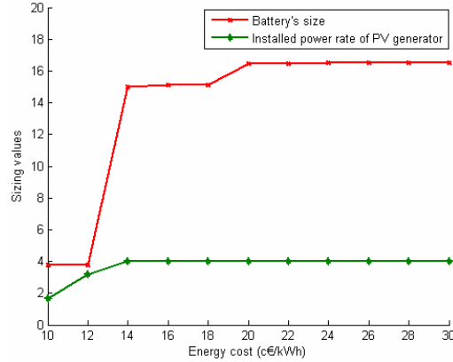
Figure 20. Correlation between PV generator and battery size.
