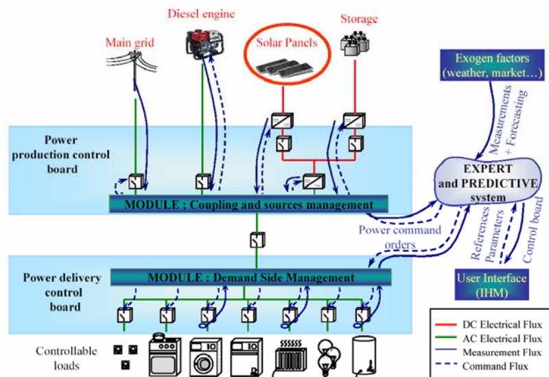
Figure 1. Optimal multi-sources and loads co-management system architecture.
