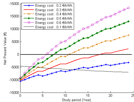
Figure 16. Net Present Value.
