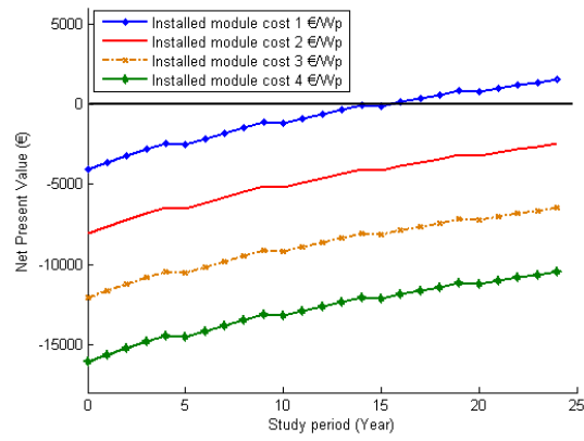
Figure 12. Net Present Value.
