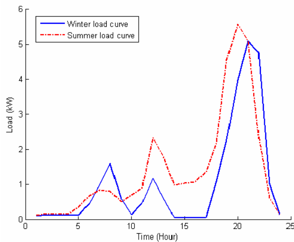
Figure 6. Load consumption curves.
