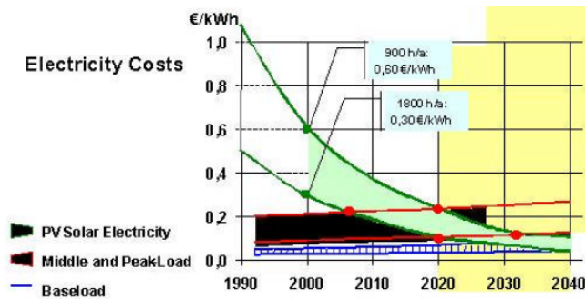
Figure 5. Cost of PV generation and electricity price evolution [1].
