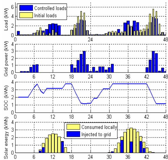
Figure 15. Operation plan (for installed module cost of 1.2 €/Wp).
